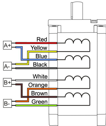
SM8680 – parallel connection
