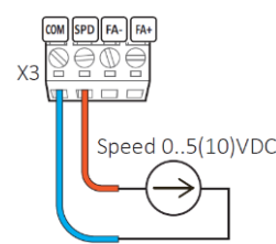
Fig. 7b. Examples of connecting an external analog signal input - speed regulation by an external voltage source
