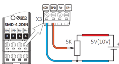
Fig. 7a. Examples of connecting an external analog signal input - speed adjustment with an external potentiometer
