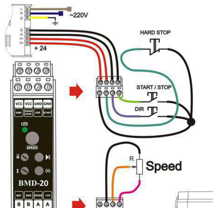
Fig.2. BMD-20DIN connection scheme (example of speed control by external potentiometer.)
