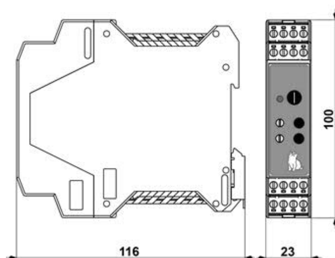
Fig.1 Dimensions of BMD-20DIN
